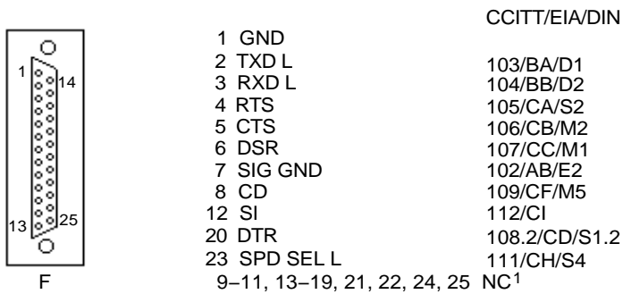
Figure B-1 Comm1 and Comm2—Serial Communication/Printer Ports
