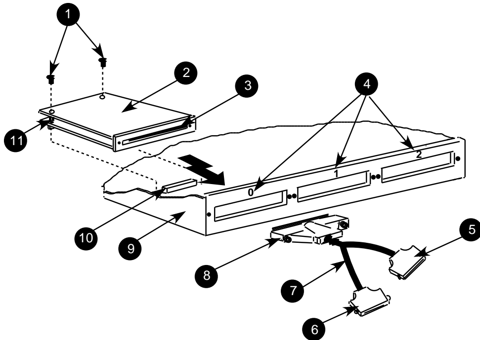
Figure 2-1: DEC WANcontroller 720 Kit Installation
